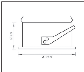
A - Ø82 X 56mm / Cutout Ø72mm
