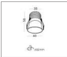
A - Ø40 X 58mm / Cutout Ø35mm
