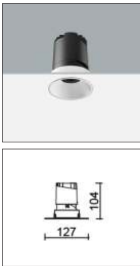
A - Ø127 X 104mm Cutout 75X104mm
