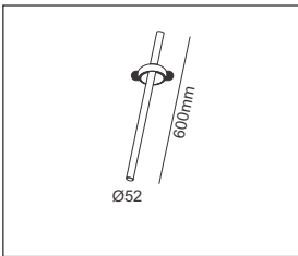
A - Ø52 X 600mm Cut out - 105mm
