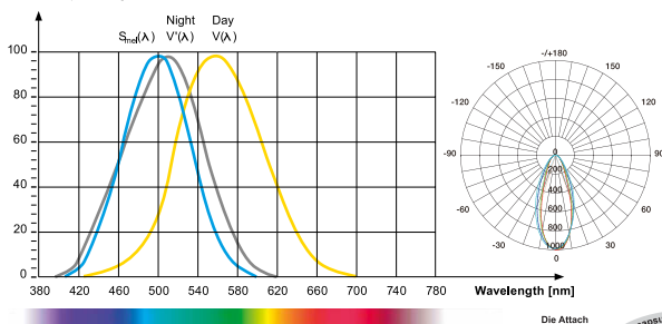
Relative spectral perception of brightness and melanopic effect Effect as a percentage
