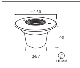
A - Ø150 X 90H mm - Cutout 110
