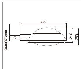
Head- Ø665 X 250Hmm
