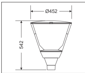
Head- Ø452 X 542Hmm
