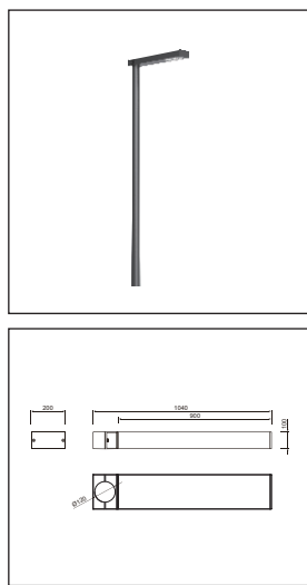
A - Ø120 x 200 x 1040mm
